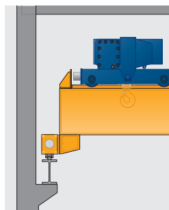
Stooped up configuration Version 4
