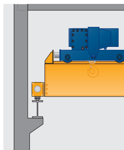
Stooped up configuration Version 3
