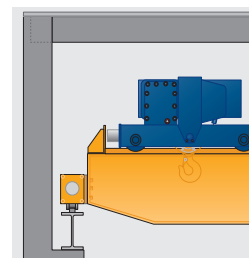
Stooped up configuration Version 2
